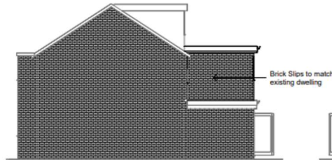
Side Elevation 1 - Proposed 1 : 100
